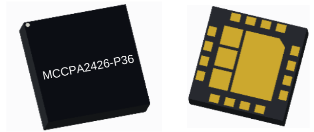
16Pad 5×5mm Laminate Package
