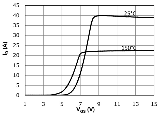
Fig 3: Transfer Characteristics
