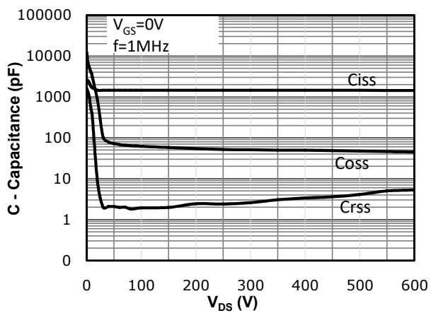
Fig 11: Capacitance Characteristics
