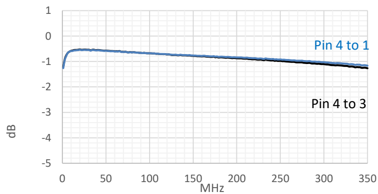
Insertion Loss
